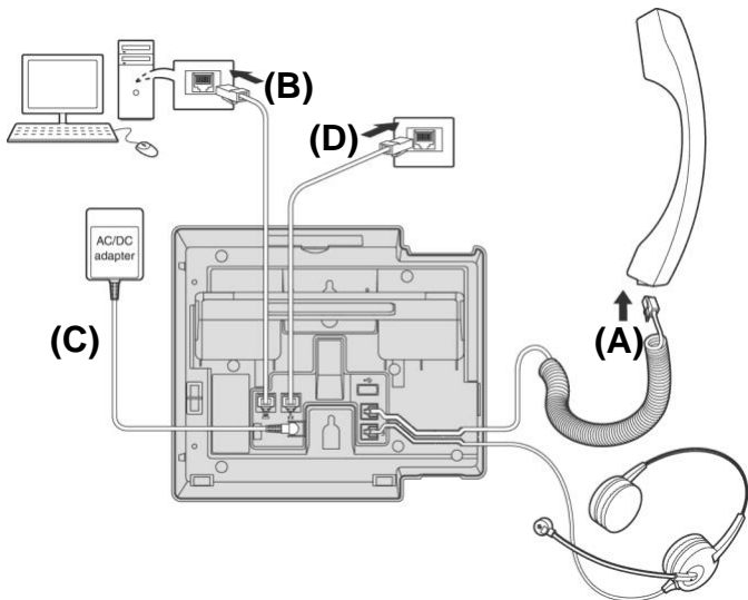
iPECS LIP-8040L Connections
